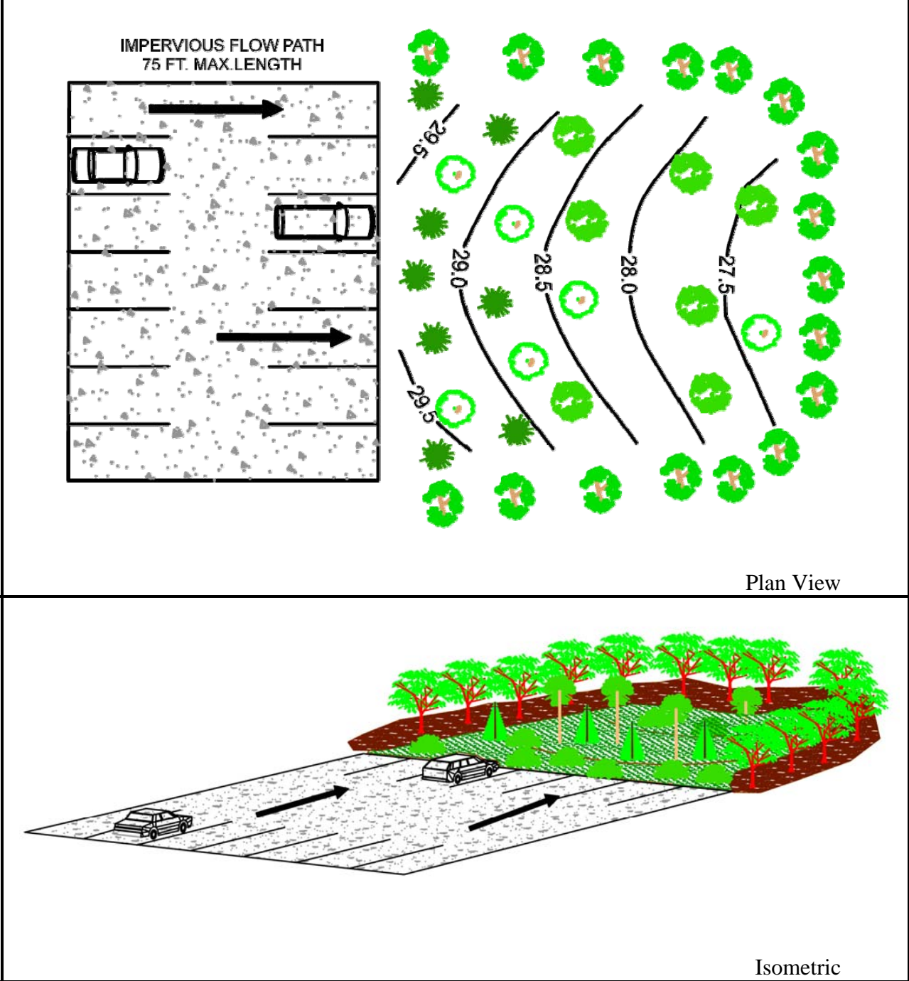
Figure 5.6 Non-Rooftop Disconnection
